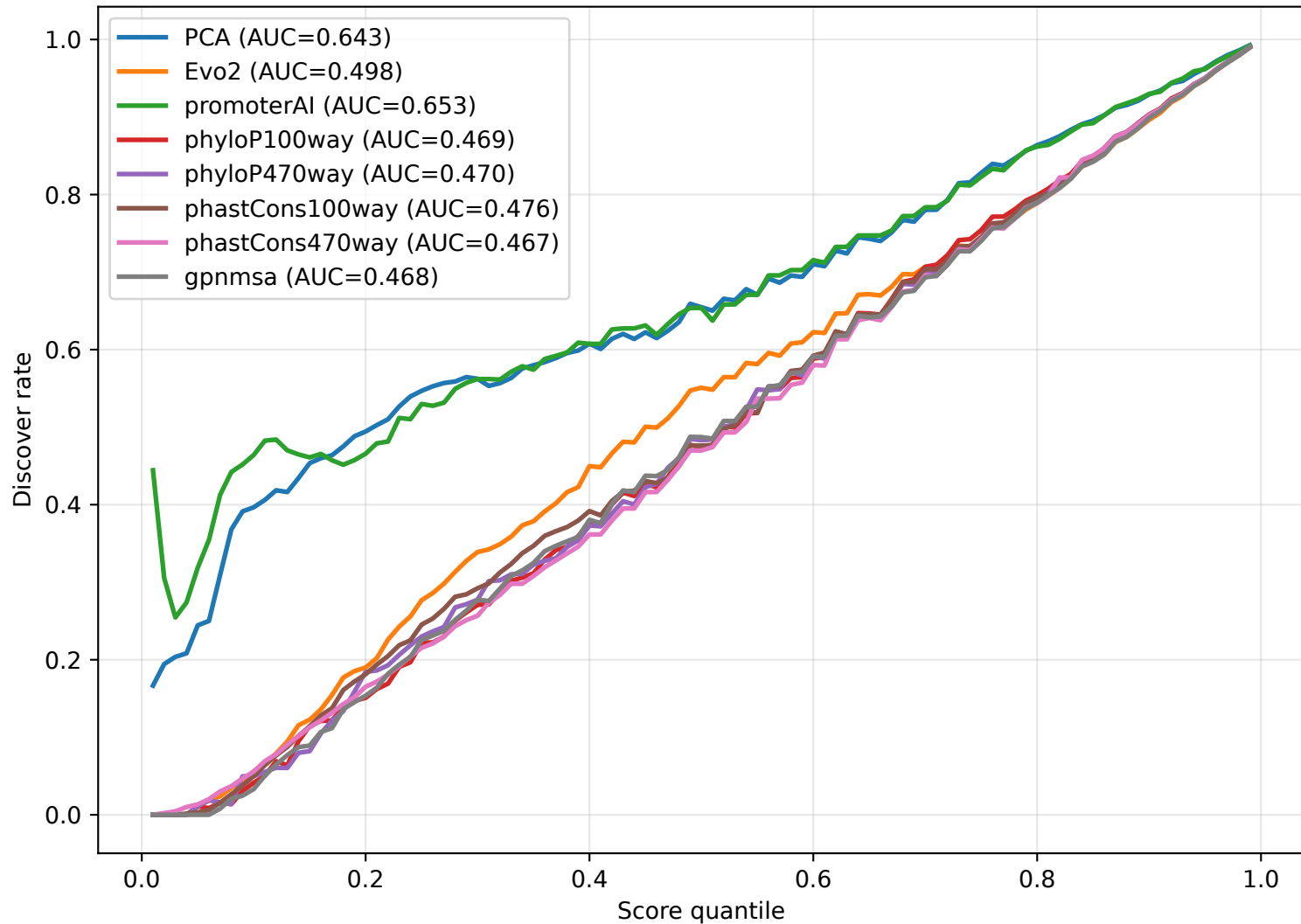
Quantile-aligned Discover Rate — SORT1
