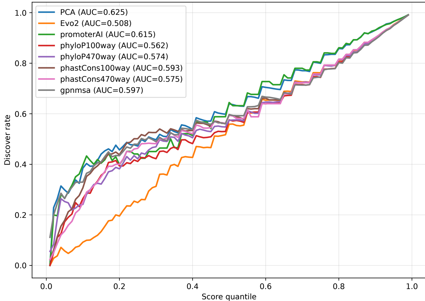
Quantile-aligned Discover Rate — ZFAND3
