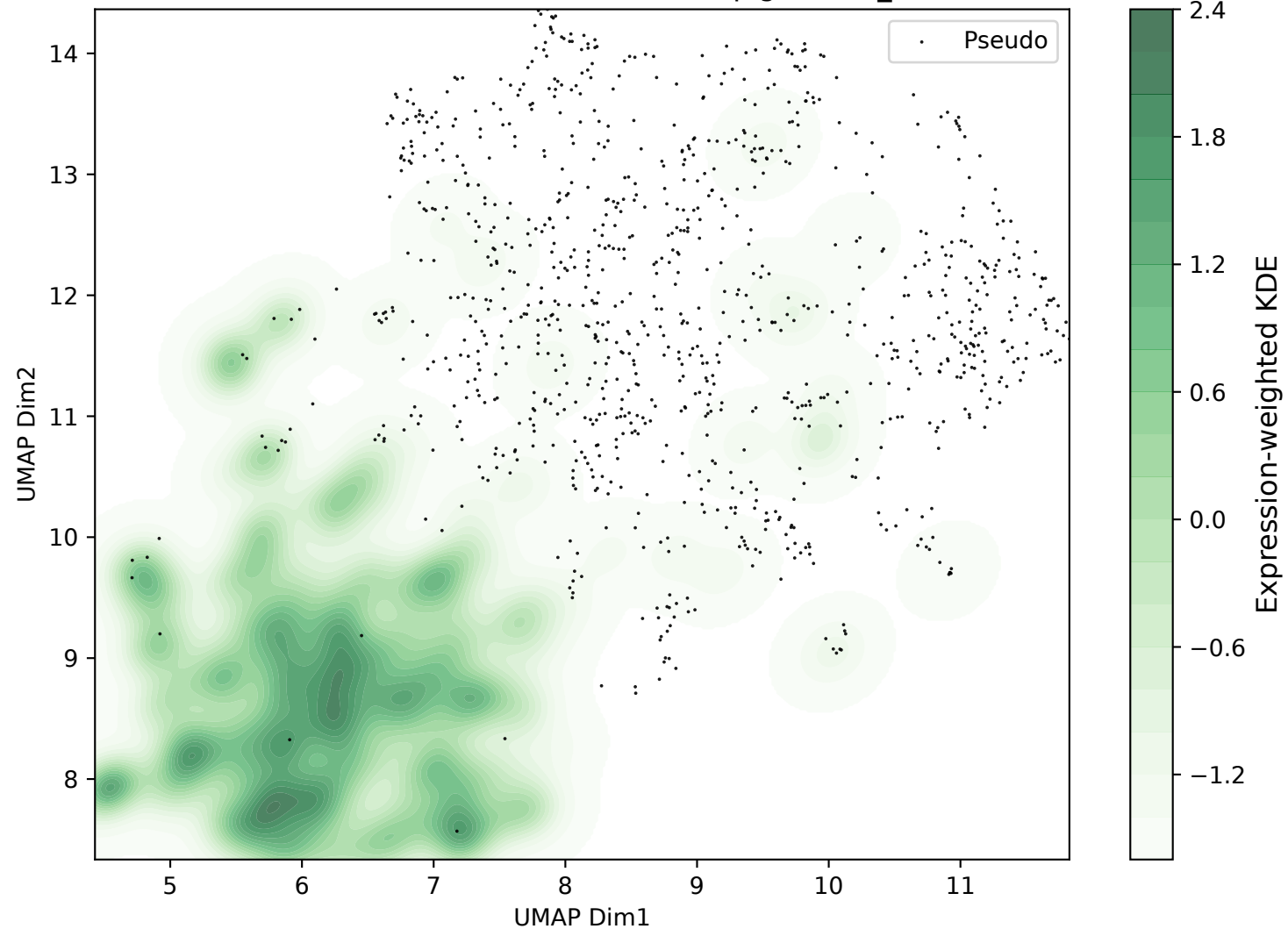
UMAP (fit on Pseudo, contour real) - epigenetics_ETF1
