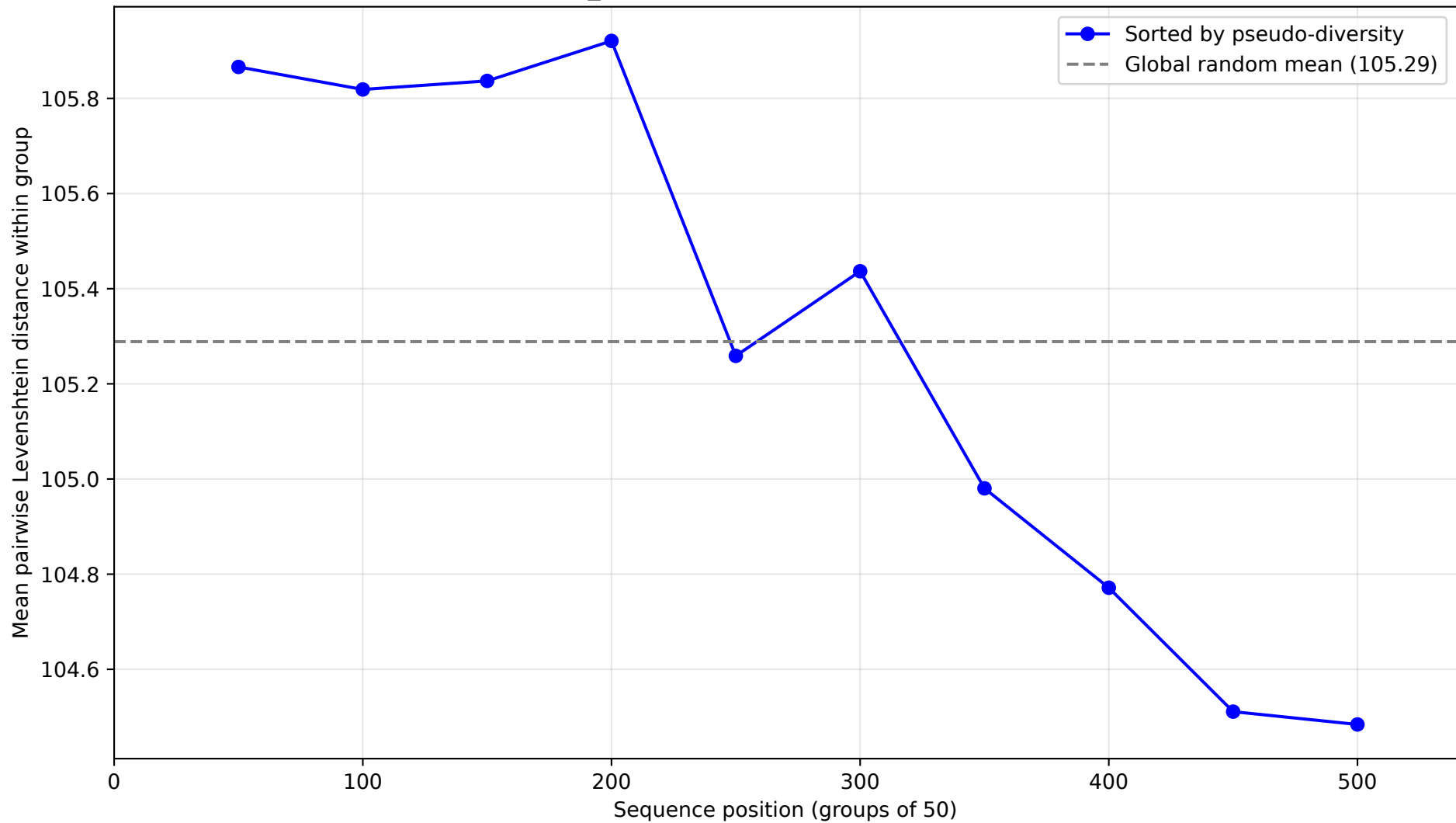
mpira_K562 — Levenshtein Distance Trend
