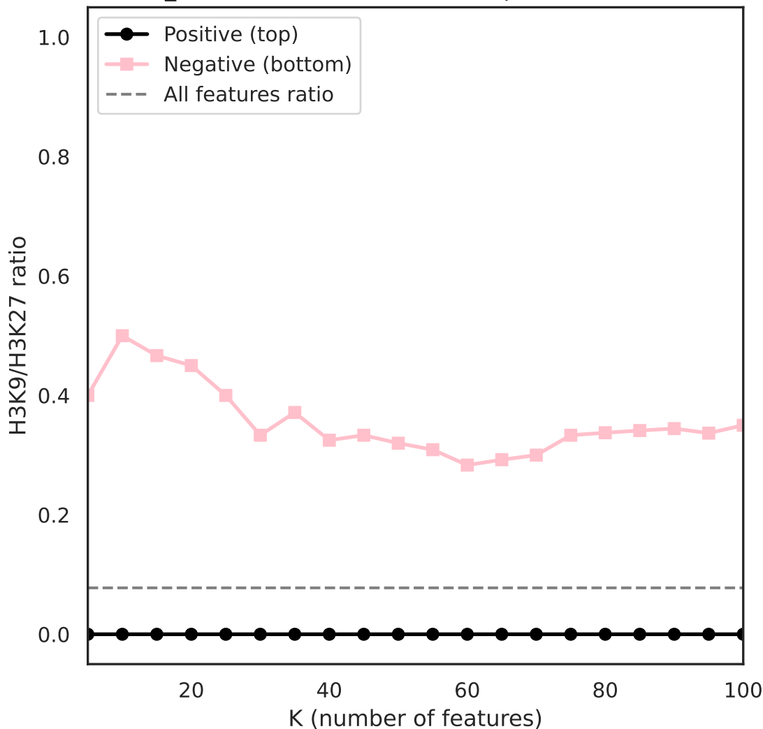
MPRA_K562 H3K9/H3K27 ratio vs Top/Bottom K features
