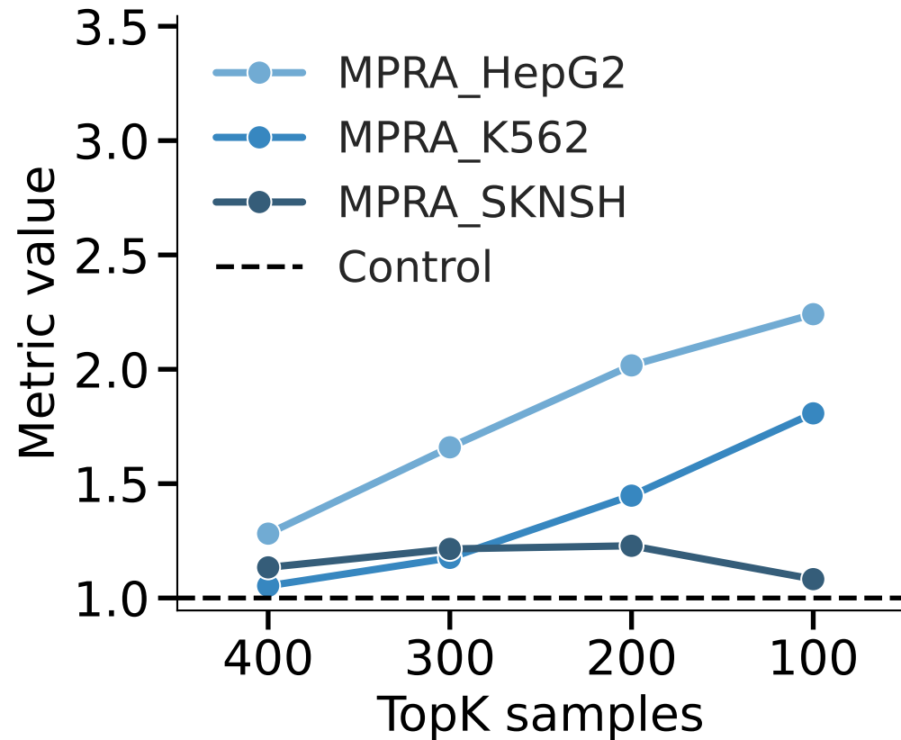
Filter_Efficiency - MPRA
