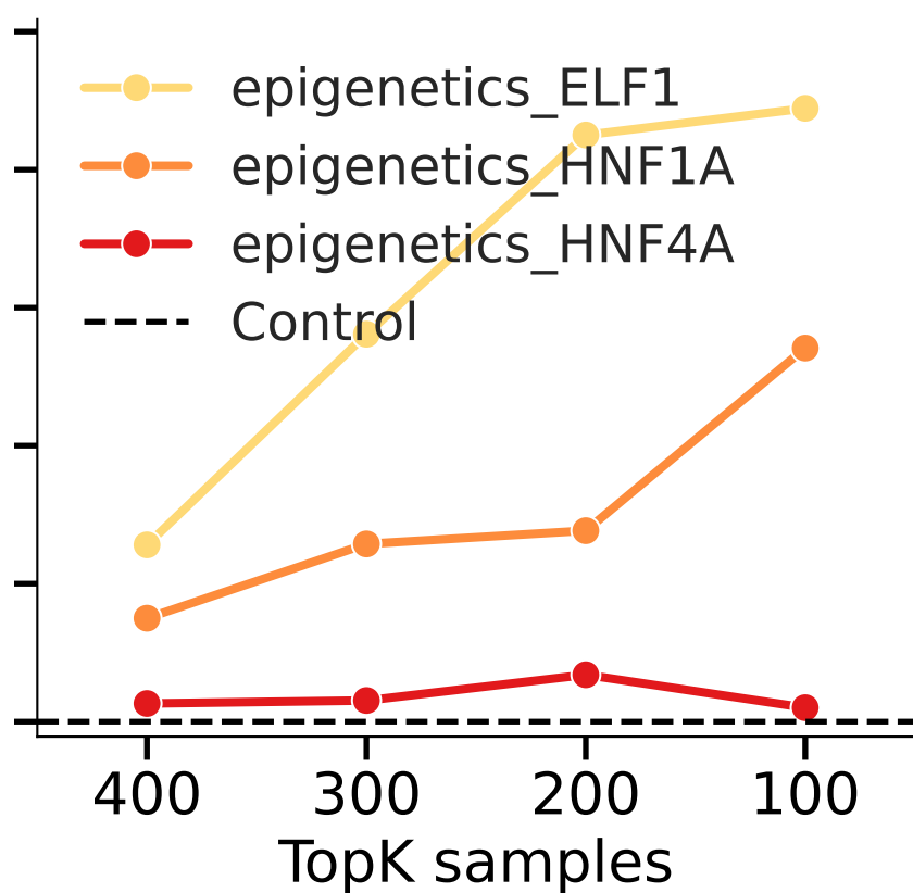
Filter_Efficiency - Epigenetics
