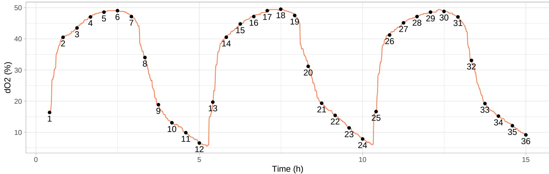
Oxygen concentrations of transcriptome of Tu et al. 2005
