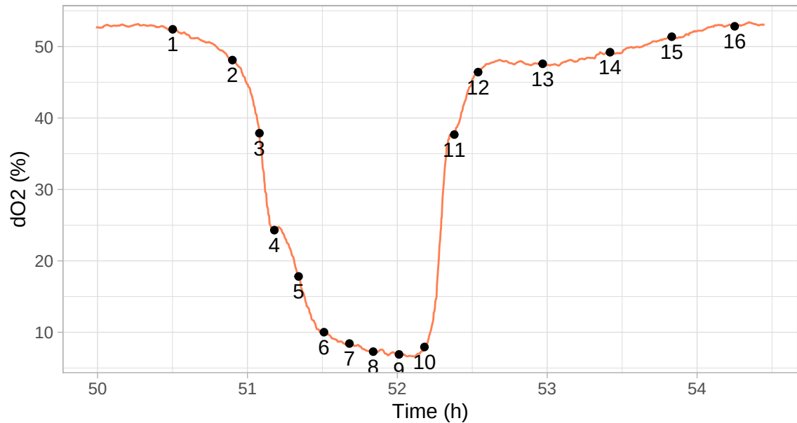
Oxygen concentrations of epigenome
