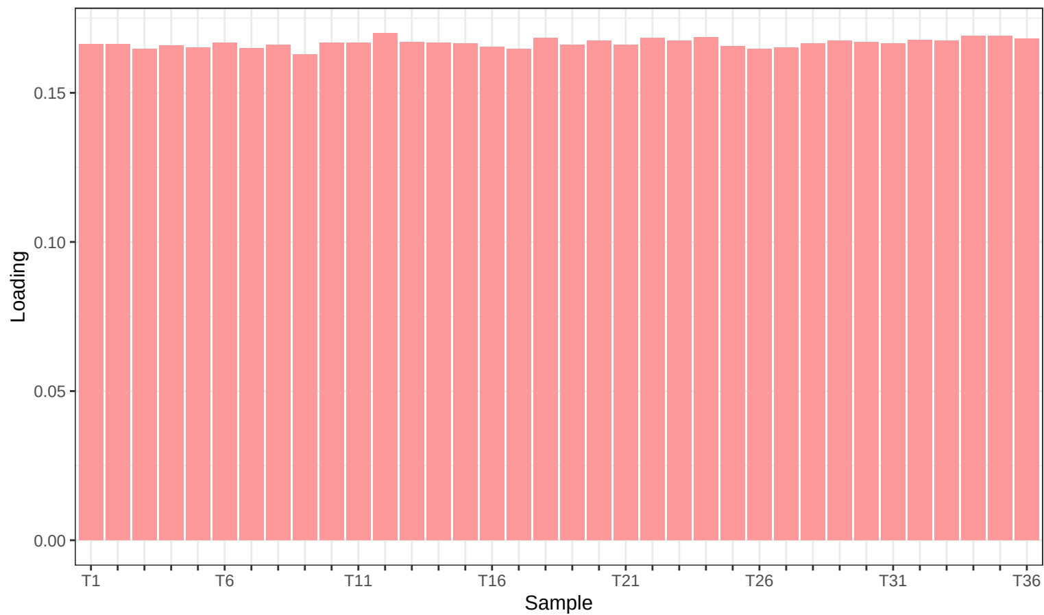
Transcriptome from Tu et al. 2005 (Level 0)
