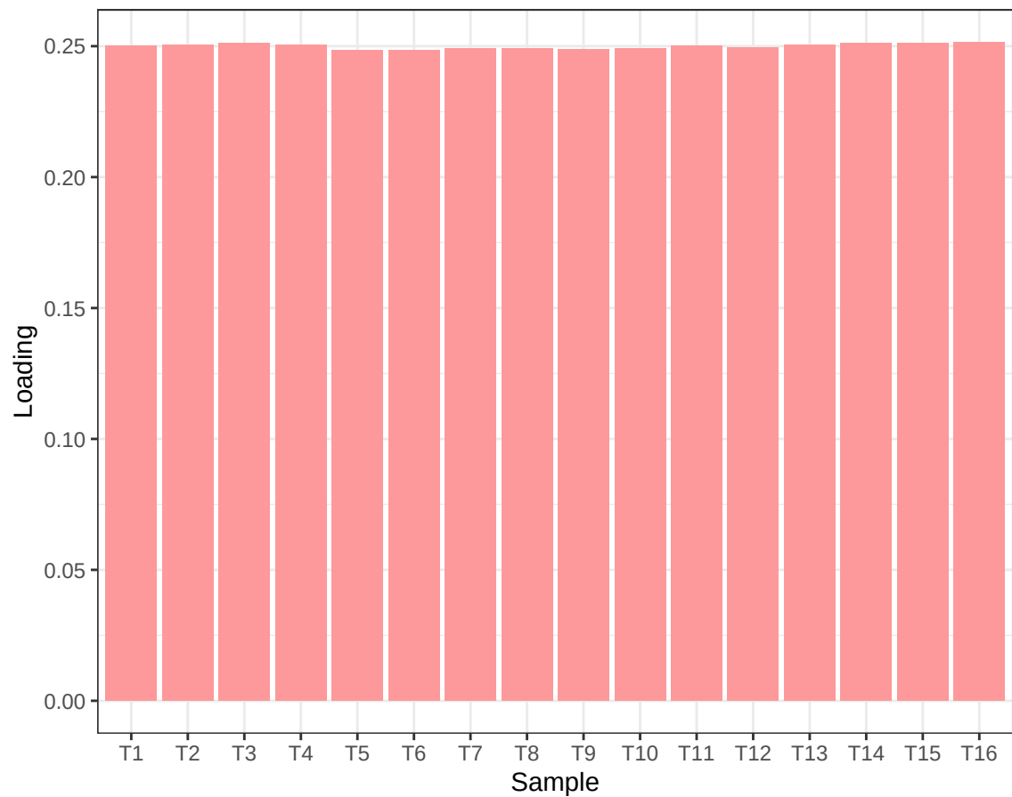
Transcriptome from Zheng et al. 2014 (Level 0)
