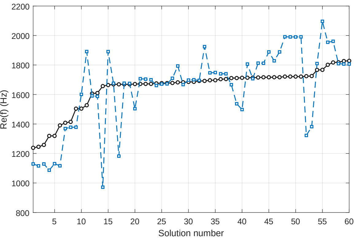
No-loss eigenmodes: COMSOL vs MATLAB
