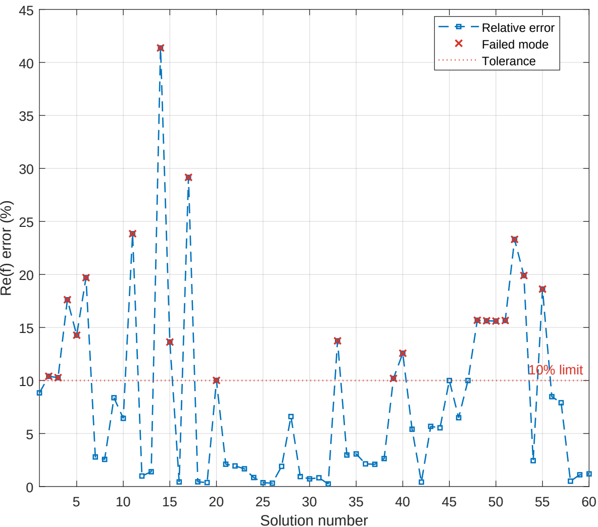
No-loss eigenmodes: COMSOL vs MATLAB — relative error
