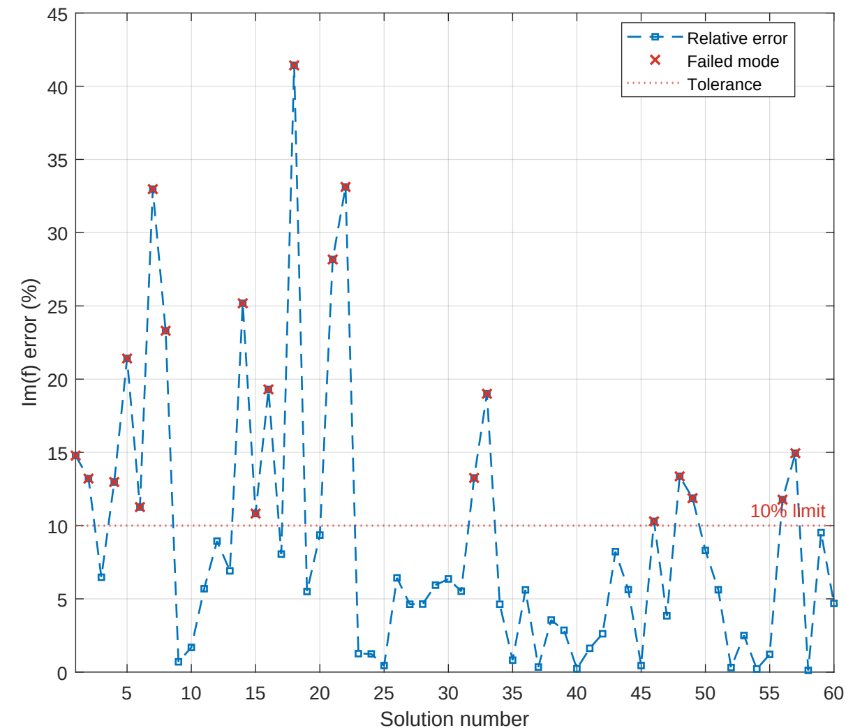
No-loss eigenmodes: COMSOL vs MATLAB — relative error
