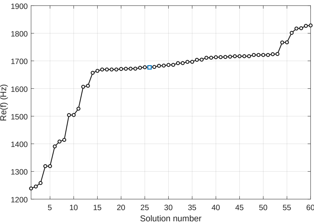
Single sector cavity 2: COMSOL TXT vs analytic mode matching
