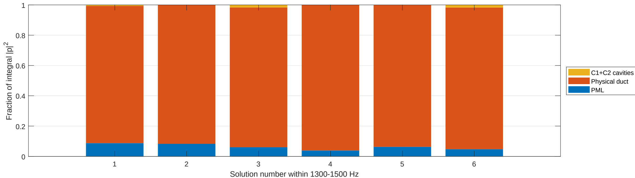
COMSOL modes in 1300-1500 Hz: pressure-energy localization
