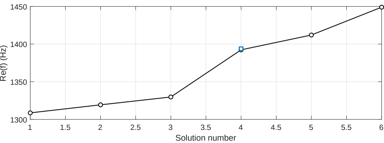
Selected C1+C2 domains (-z layer): COMSOL versus analytic MATLAB (1309-1449 Hz)
