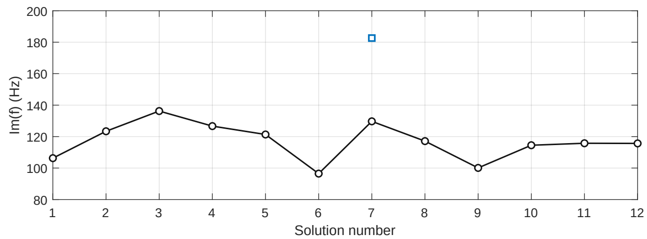
Selected C1+C2 domains (-z layer): COMSOL versus analytic MATLAB (<1600 Hz)
