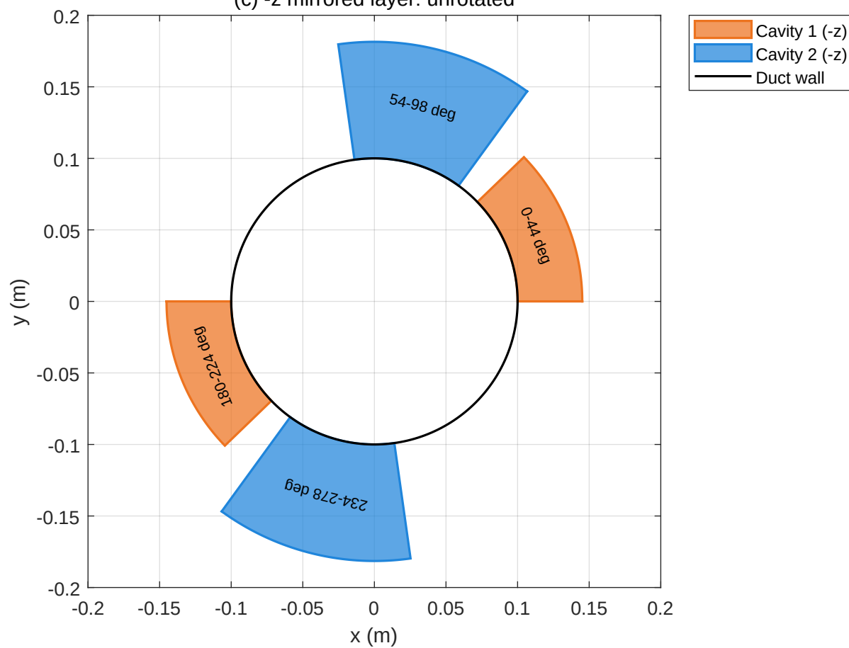
(c) -z mirrored layer: unrotated
