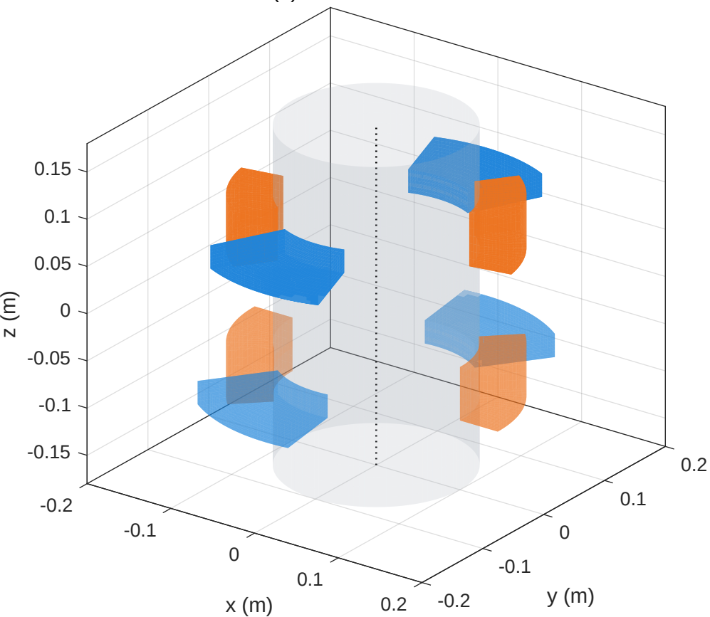
(a) Active 3D structure
