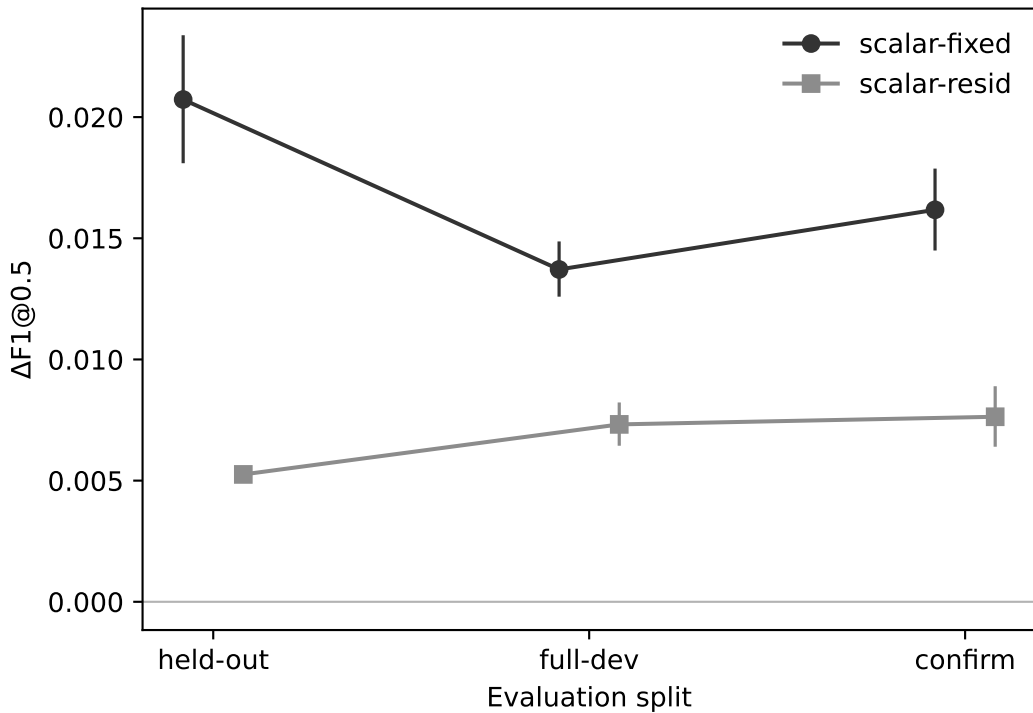
Effect replication across splits
