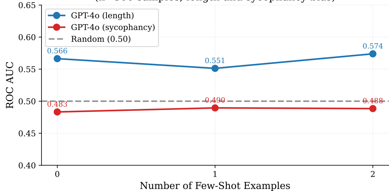
Figure 11b: GPT-4o Bias Detection vs Few-Shot Count (n=500 samples, length and sycophancy bias)
