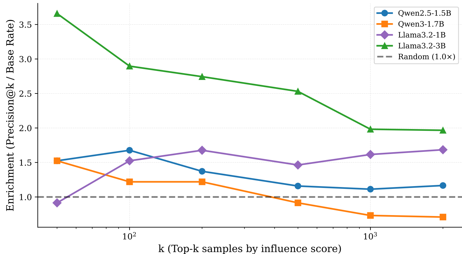
Figure 13: Top-k Suspicious Sample Detection Enrichment over Random Baseline — Llama-3.2-3B Achieves 3.7\times at k=50
