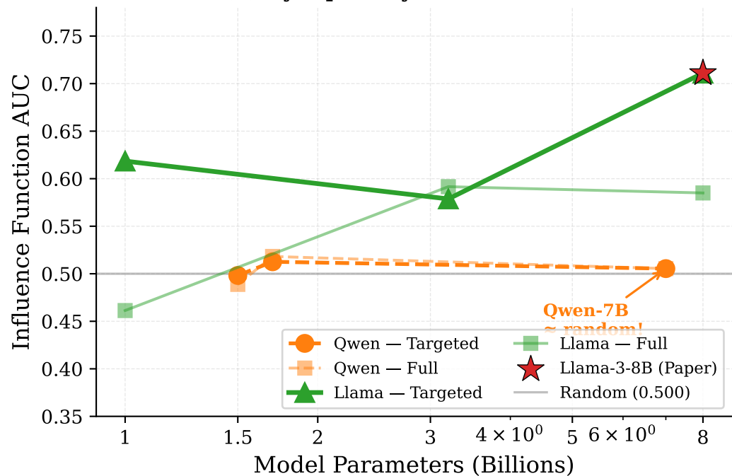
(b) Sycophancy Bias Detection
