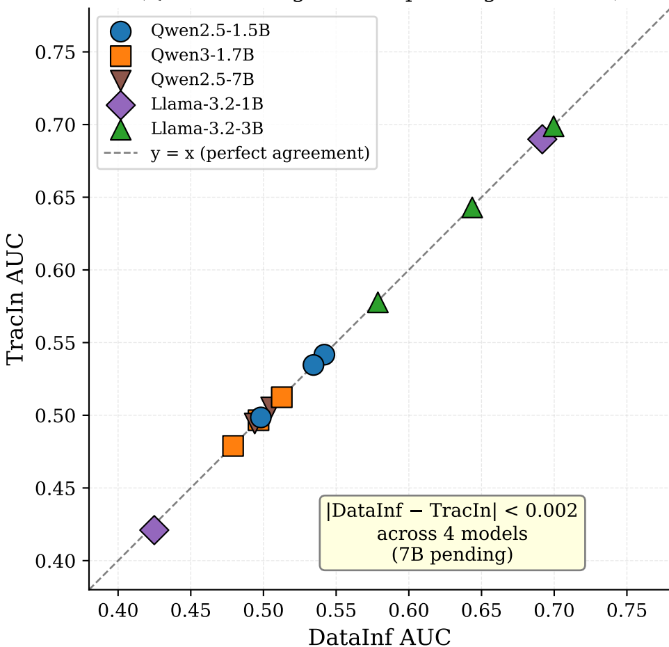
Figure 5: DataInf \approx TracIn Across All 4 Available Models (Qwen2.5-7B grad files pending download)
