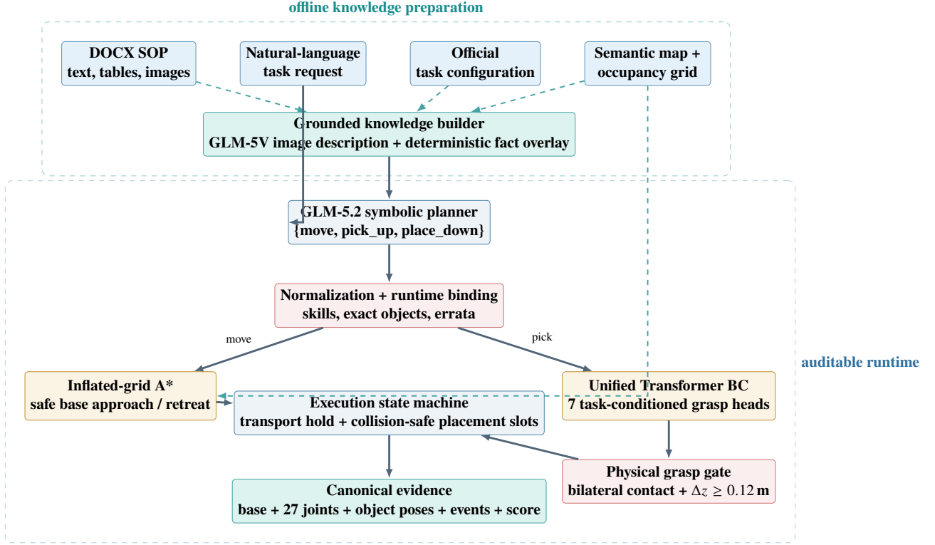
Figure 1. System overview. Language models are restricted to knowledge extraction and symbolic planning; deterministic guards bind plans to official scene identities. Continuous grasping is delegated to BC, while physical measurements decide whether execution may transition to transport. Every cross-module decision is serialized into the trajectory evidence.
