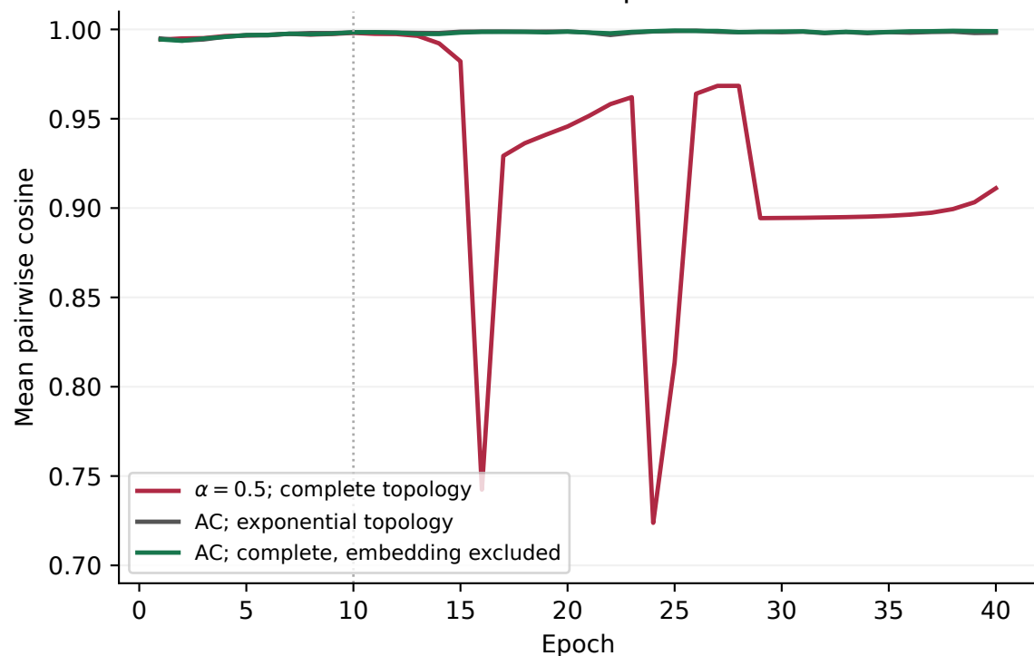
D. Residual energy migrates between tensors ( \alpha = 0.5 )
