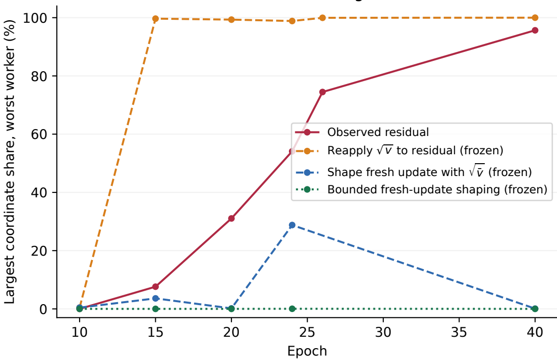
C. Error concentrates in single coordinates
