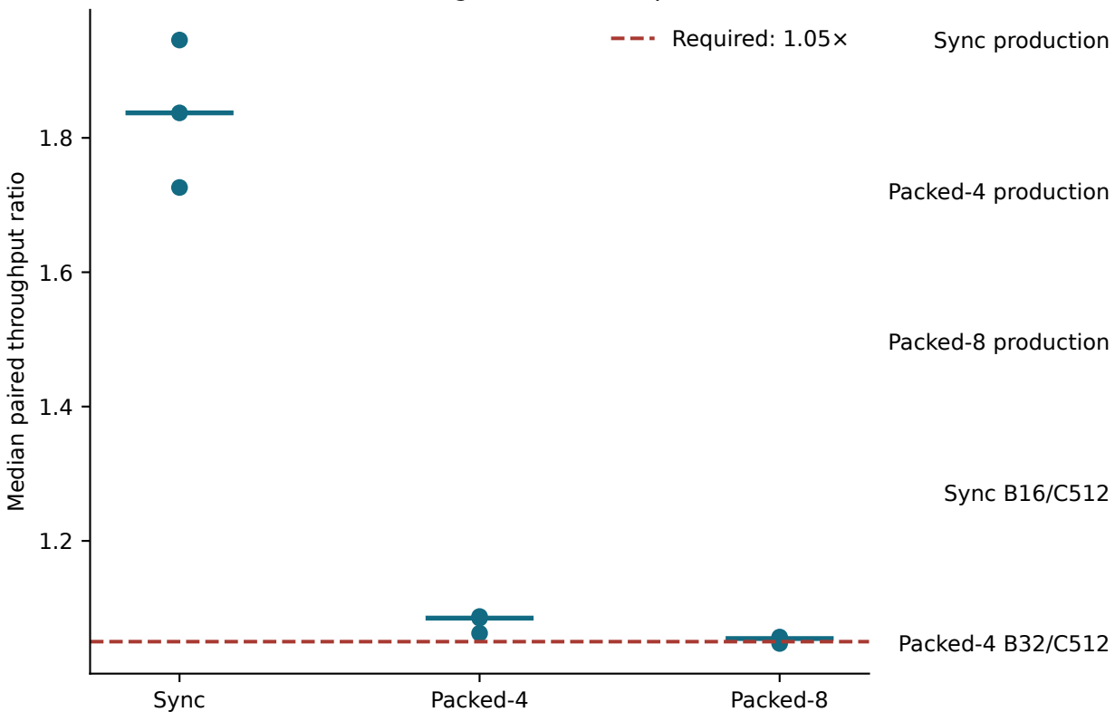
Small-batch categories: three repeats
