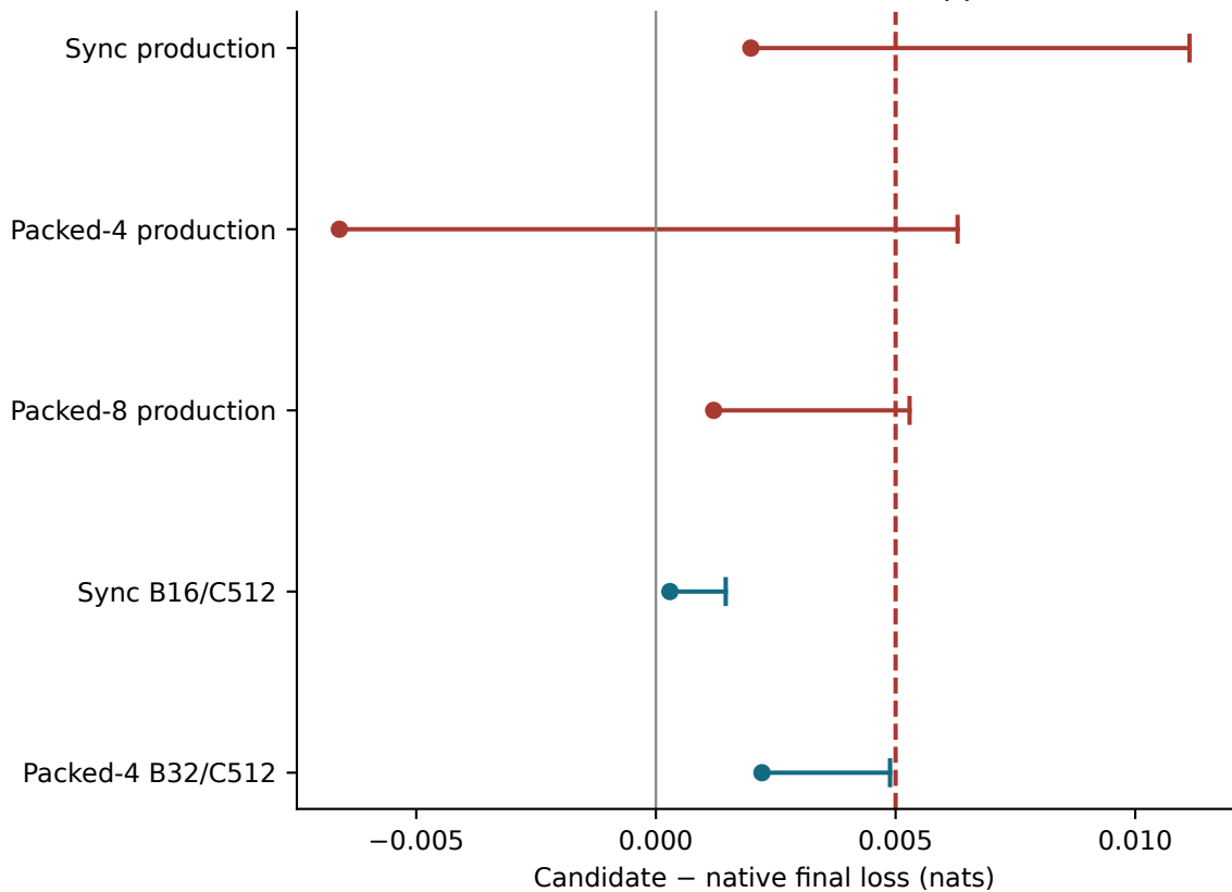
Paired mean and one-sided 95% upper bound
