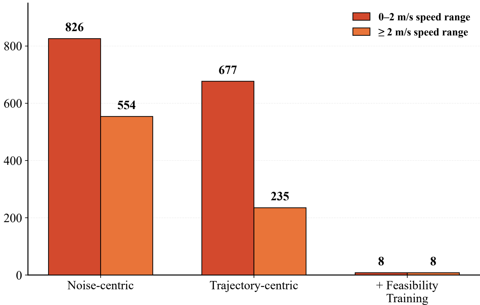
Curvature Violation Number
