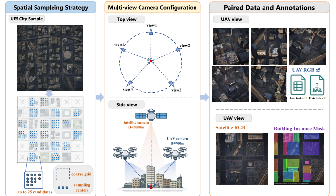
Fig. 1. Overview of the SynSU-Build sampling and rendering pipeline. Left: urban sampling uses a coarse spatial grid with up to 25 candidate centers per cell and content-based filtering. Middle: five oblique UAV cameras surround a common scene center, while one synthetic satellite-like camera observes it from nadir. Right: each accepted group contains five unannotated UAV RGB images with camera parameters and a paired satellite-like RGB image with its building instance mask.
