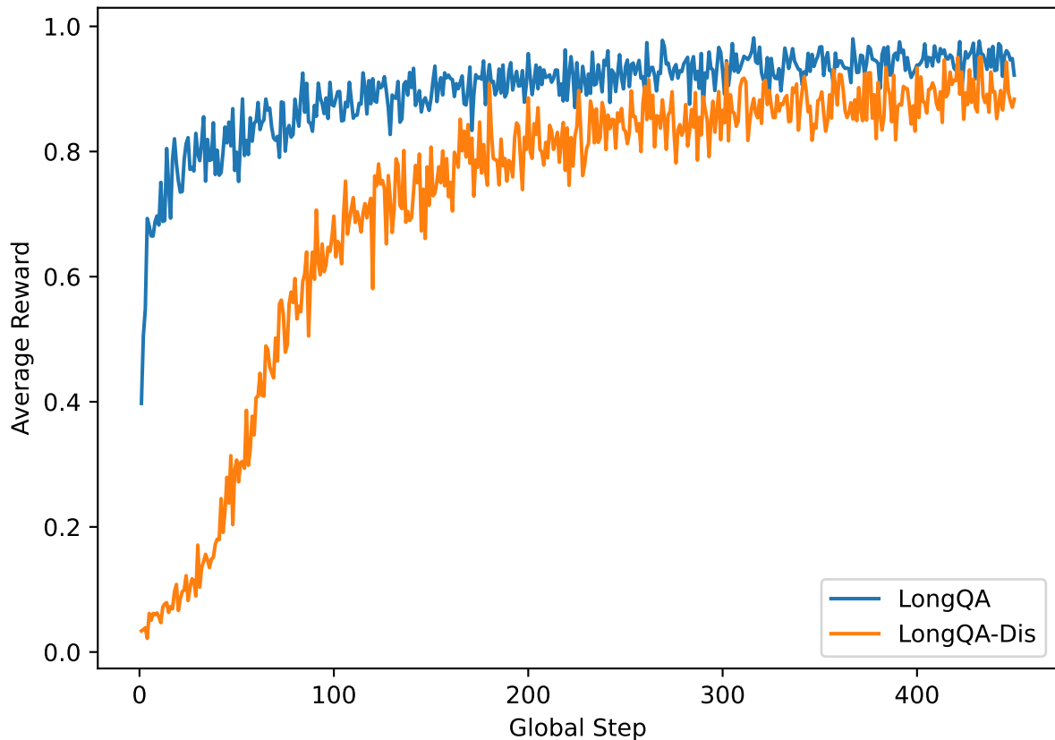
Average reward across steps
