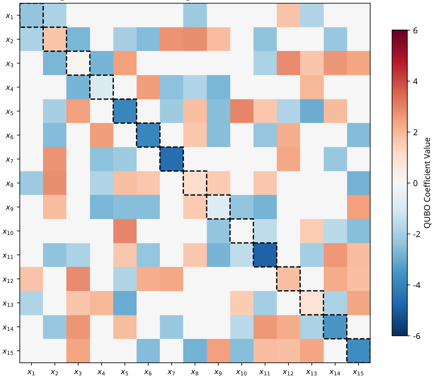
Illustrative QUBO Matrix Q for MCLP Formulation (Diagonal: Linear Terms; Off-diagonal: Quadratic Interaction Terms)
