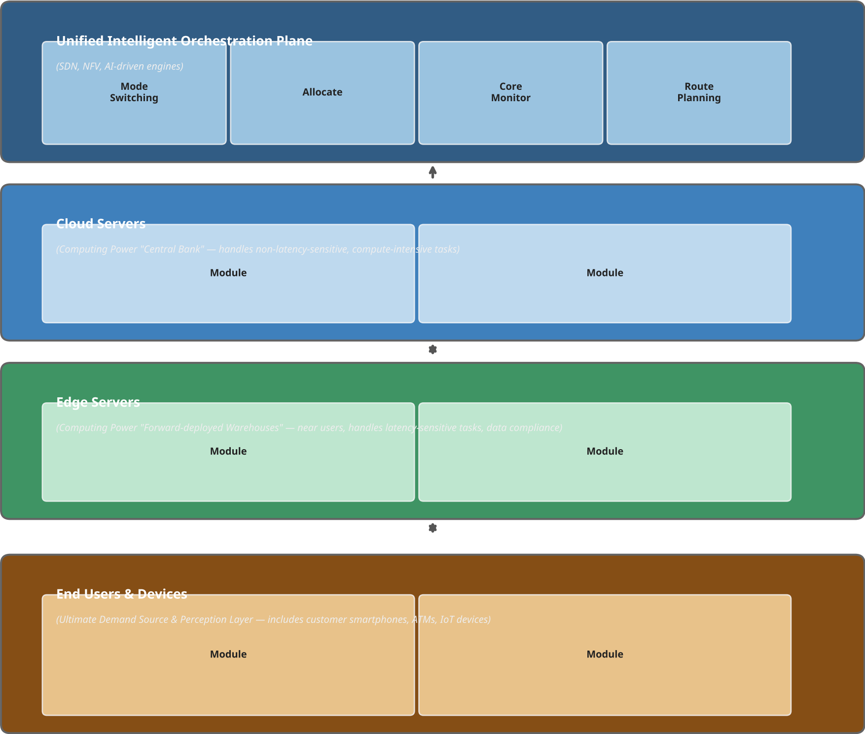
Figure 2: F-CPN Conceptual Architecture
