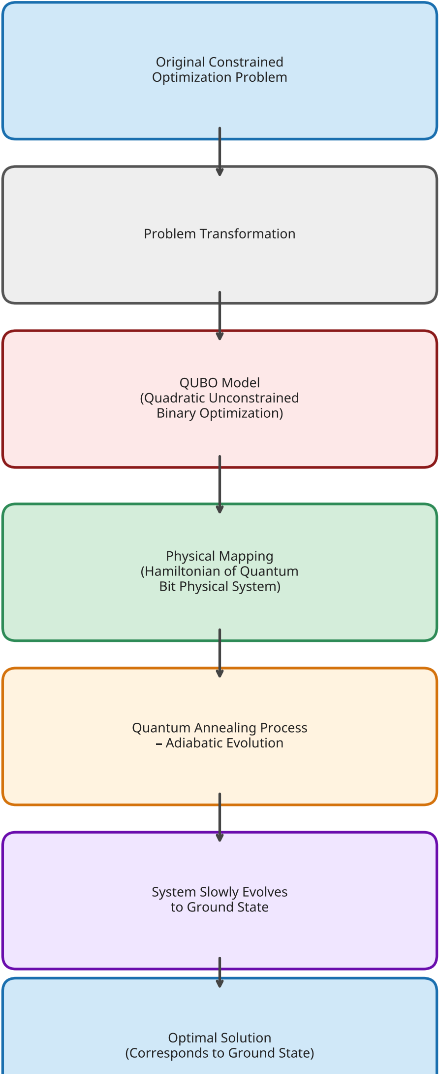
Figure 4: Process of QUBO
