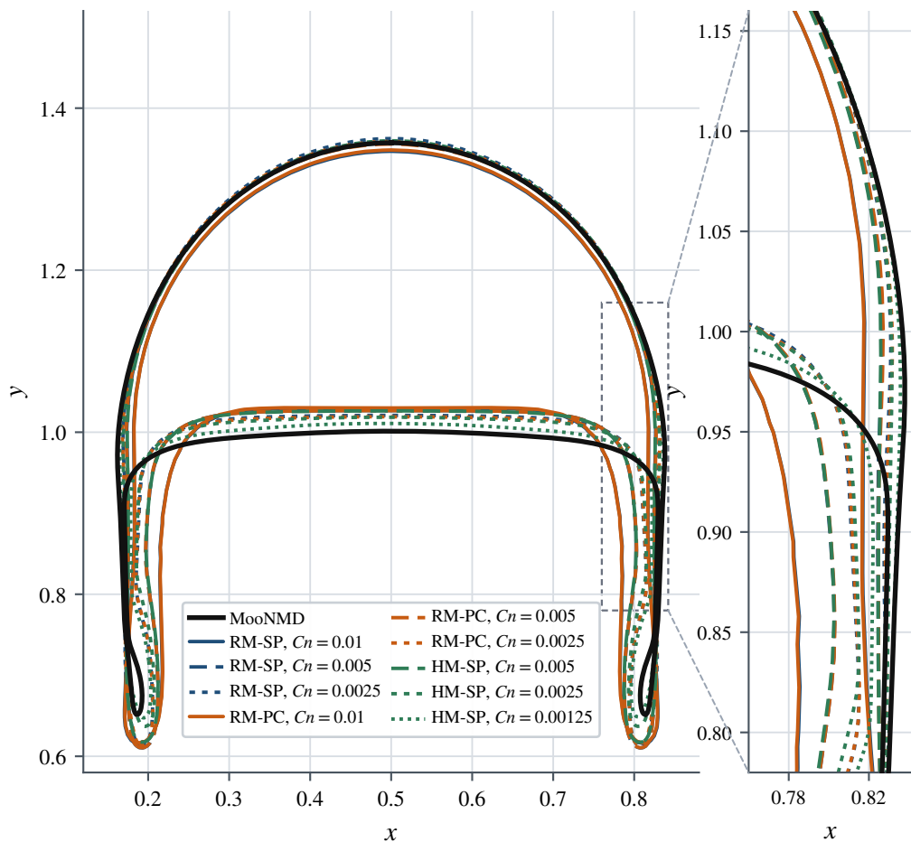
Case 2: final bubble contour ( t = 3 )
