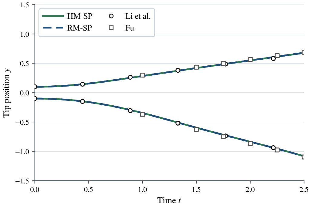
At = 0.50, Re = 3000 : bubble and spike tip evolution
