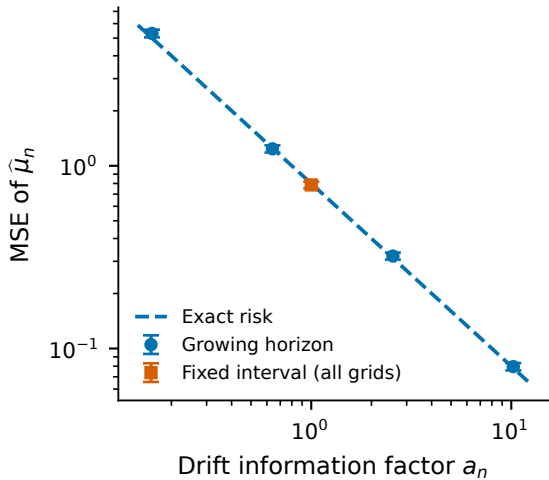
a Drift estimation
