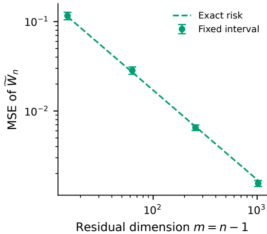
b Realized scale
