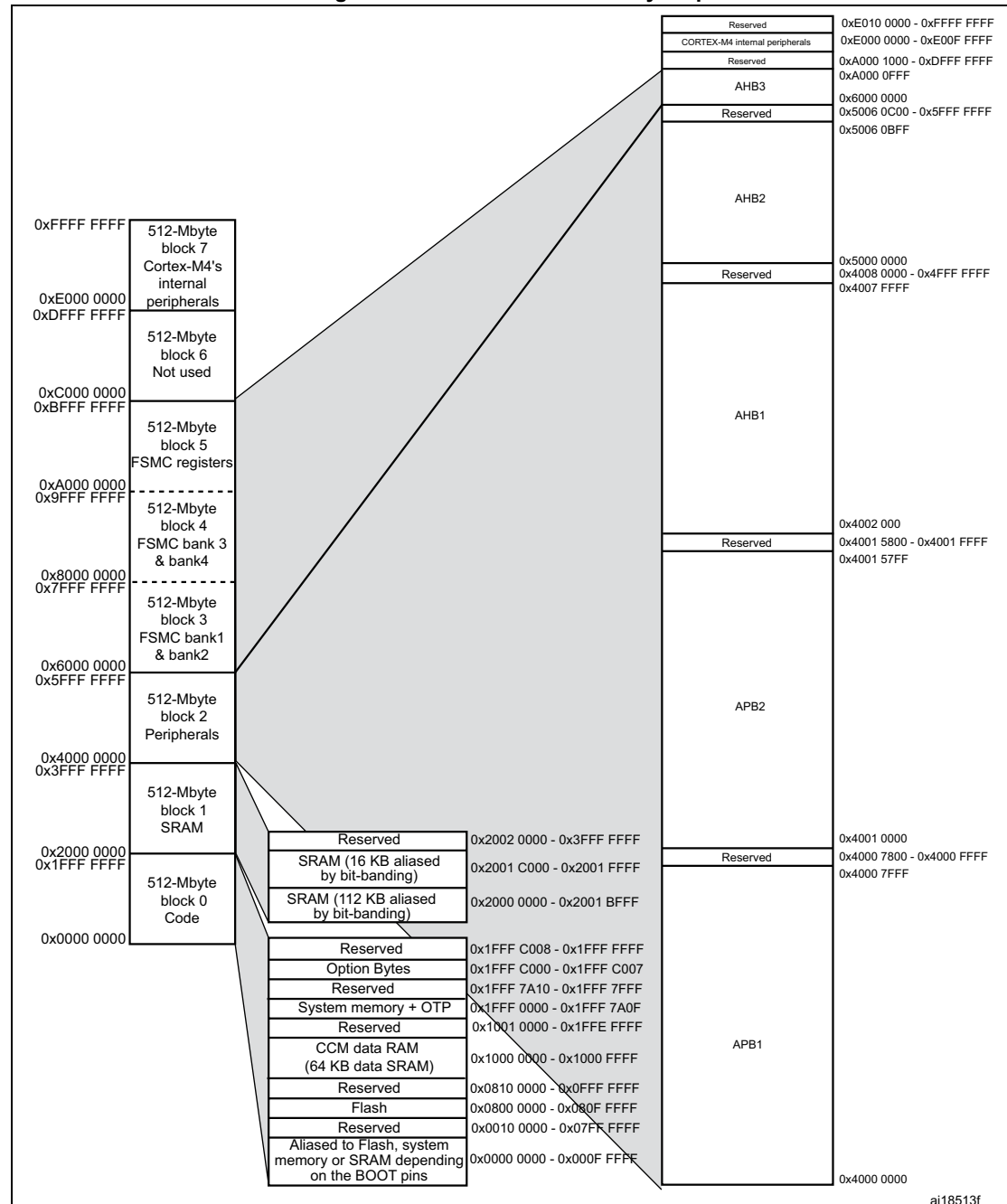
Figure 18. STM32F40xxx memory map
