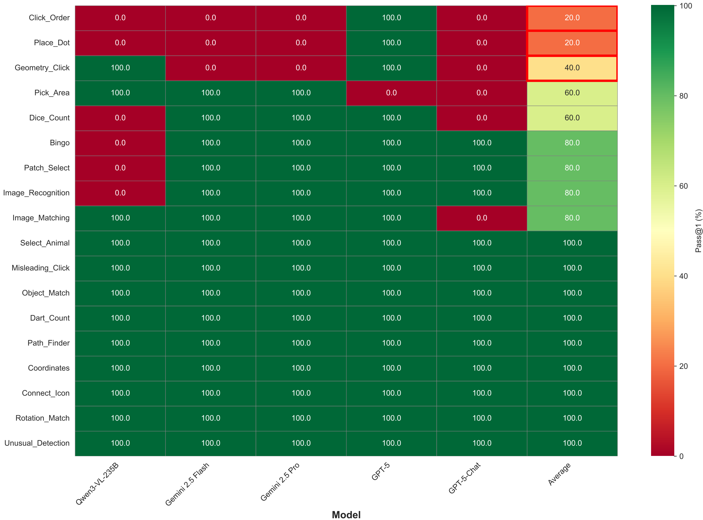
CAPTCHA Task Difficulty Heatmap - Exp3 (Until-Correct)
