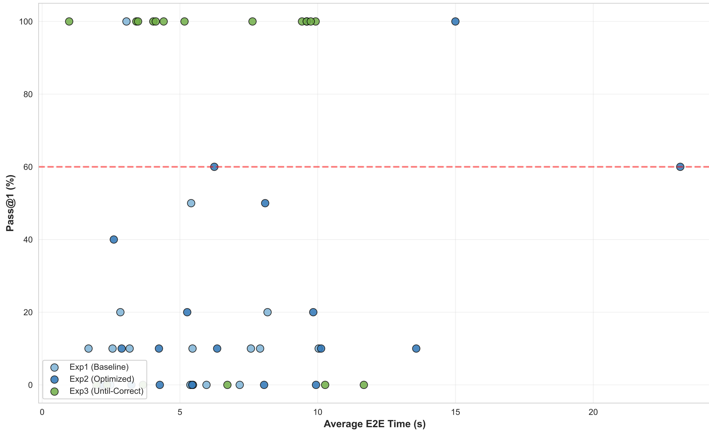
Time-Performance Scatter Model: Qwen3-VL-235B
