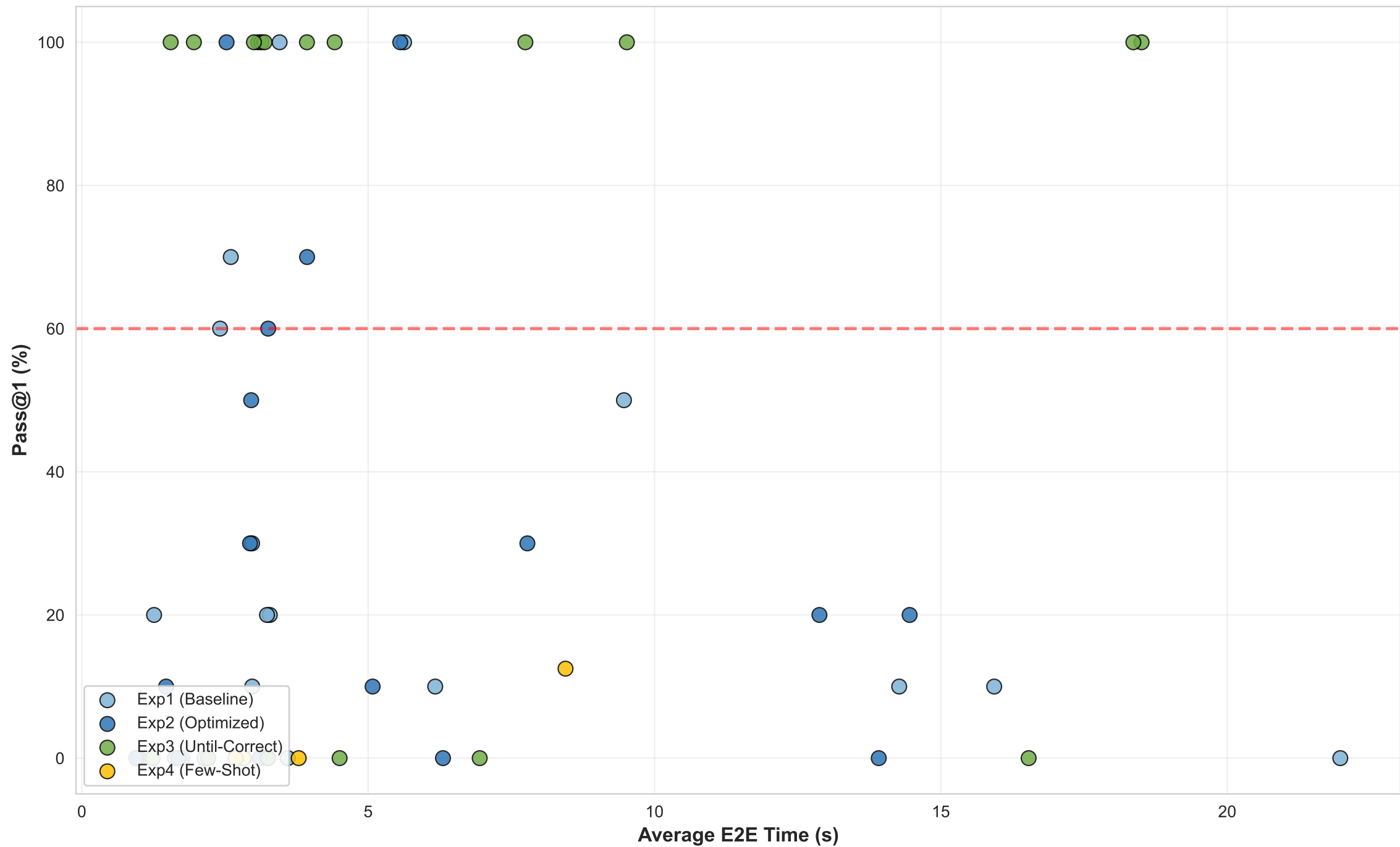
Time-Performance Scatter Model: GPT-5-Chat
