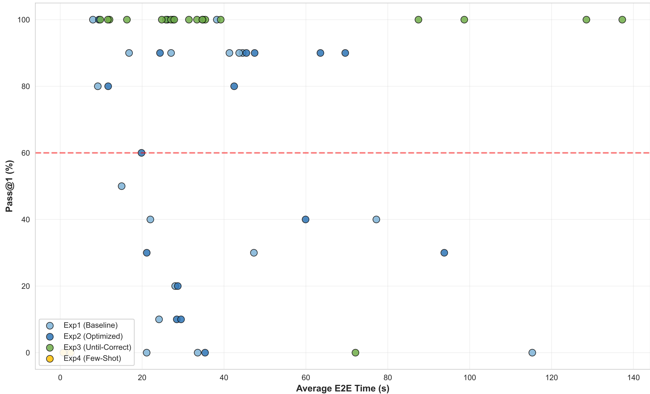
Time-Performance Scatter Model: GPT-5
