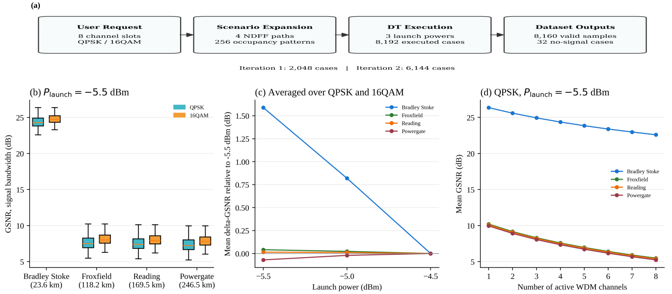
Fig. 7. GNPY-based optical QoT dataset generation over the NDFF topology. (a) Agent-driven scenario expansion and dataset-generation workflow, (b) GSNR distributions for QPSK and 16QAM over the four paths at P_{\text{launch}} = -5.5 dBm, (c) route-dependent GSNR variation with launch power, averaged over QPSK and 16QAM and normalised to the results at -5.5 dBm, (d) mean GSNR as a function of the number of active WDM channels for QPSK transmission at P_{\text{launch}} = -5.5 dBm.
