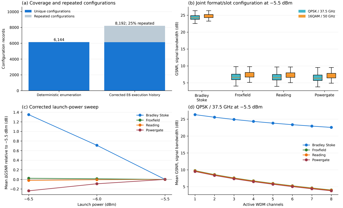
Fig. 7. GNP feasibility demonstration over the NDFF topology. (a) Configuration enumeration and execution-history counts; (b) GSNR distributions for the two modulation/slot-width settings at -5.5 dBm; (c) route-dependent mean GSNR change across the launch-power sweep; and (d) QPSK mean GSNR versus active-channel count. Numerical panels use 6,120 valid unique configurations; 24 all-off cases are excluded from metric summaries. GSNR is measured over the signal bandwidth.
