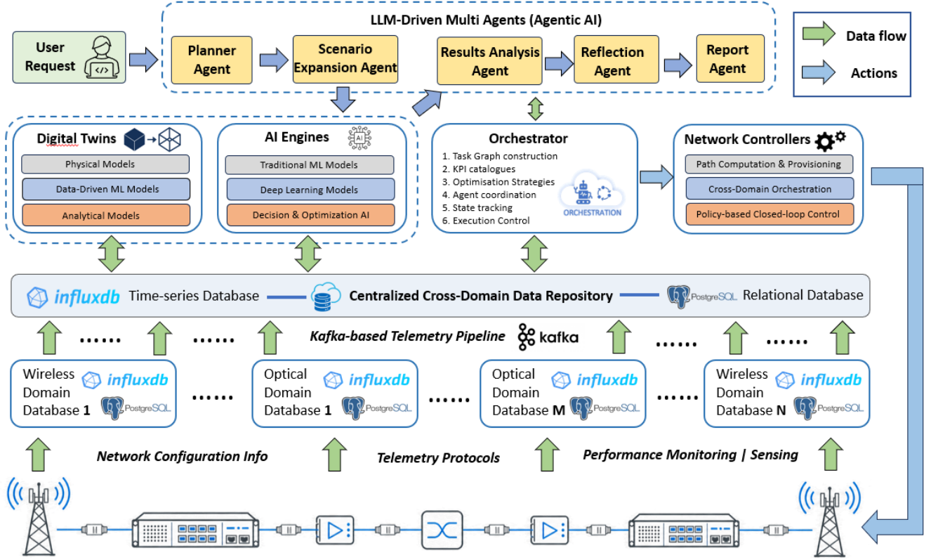
Fig. 1. Scope map of the cross-domain dataset framework, including practical data collection, semantic abstraction, and the demonstrated DT data-generation workflow.
