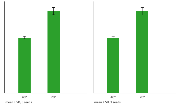
Fig. 9. Synthetic LiFi/OWC response to receiver FOV. The in-FOV fraction is computed from sampled optical states; the received-packet fraction is computed from exported LiFi flow counters. Bars show mean \pm SD across three seeds after CPE and nuisance-condition averaging.
