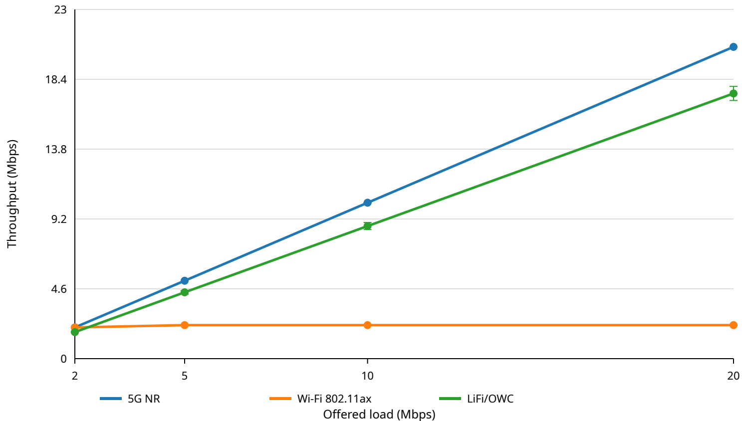
W4C synthetic wireless throughput
