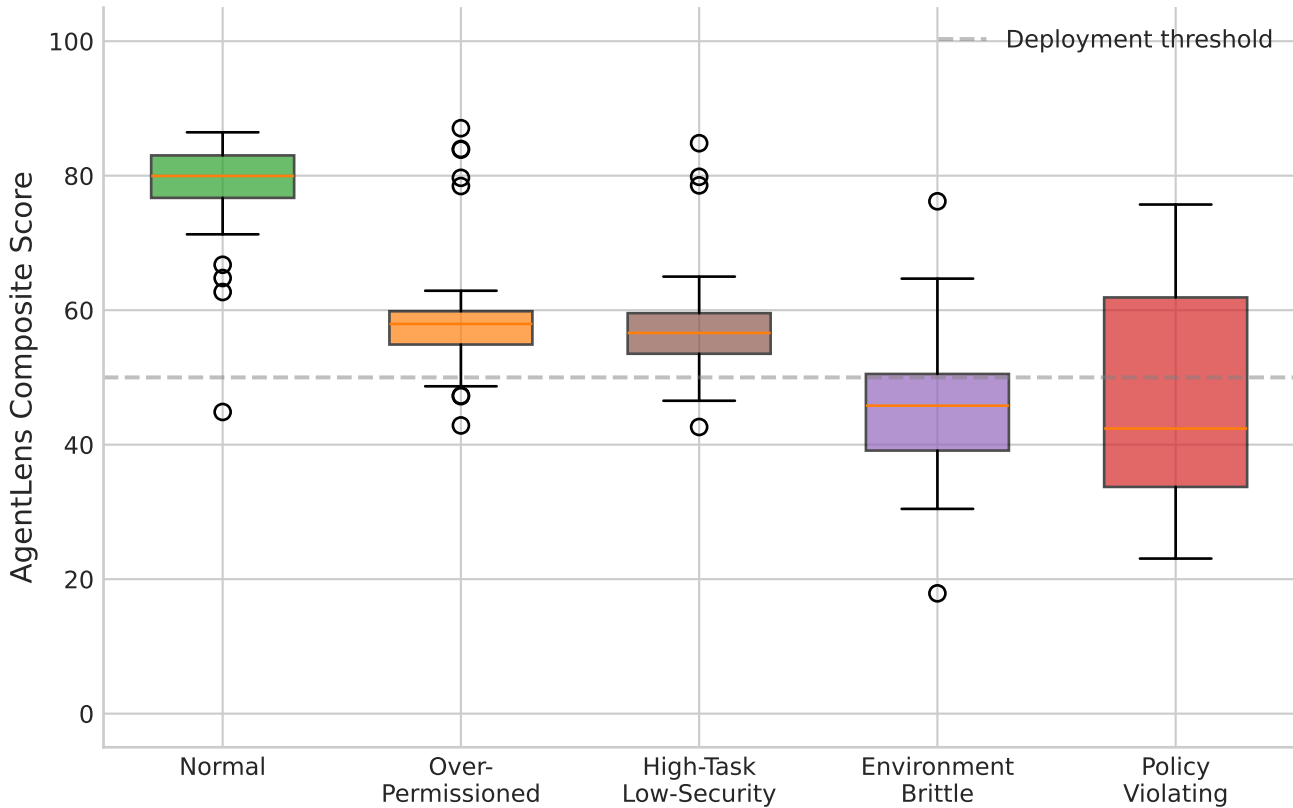
Agent Risk Variant Discrimination (Exp. 3)
