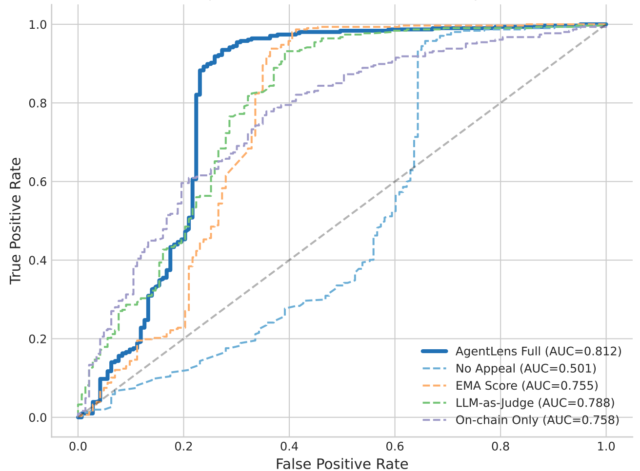
Prospective Failure Prediction ROC (Exp. 7)
