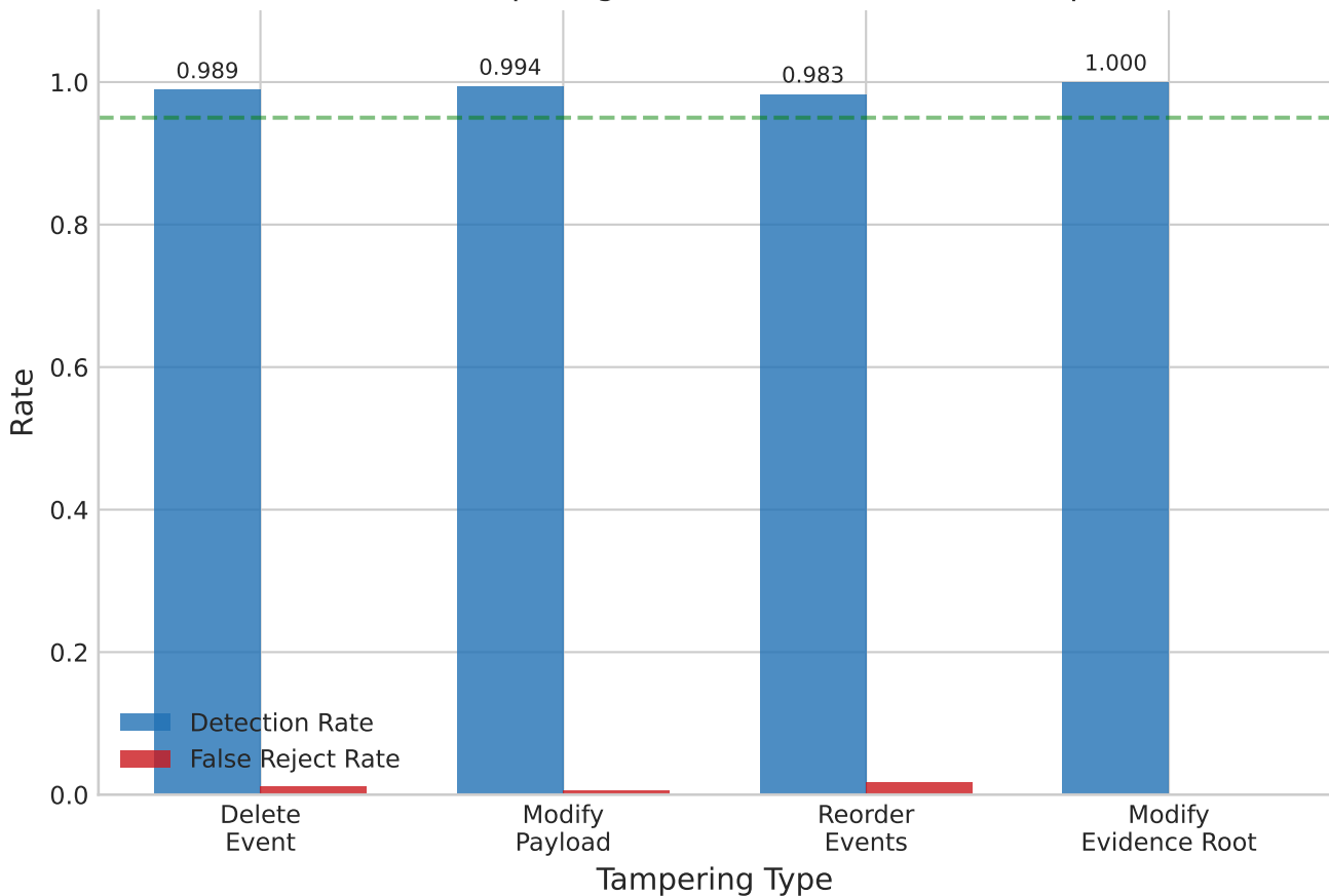
Evidence Tampering Detection Performance (Exp. 9)
