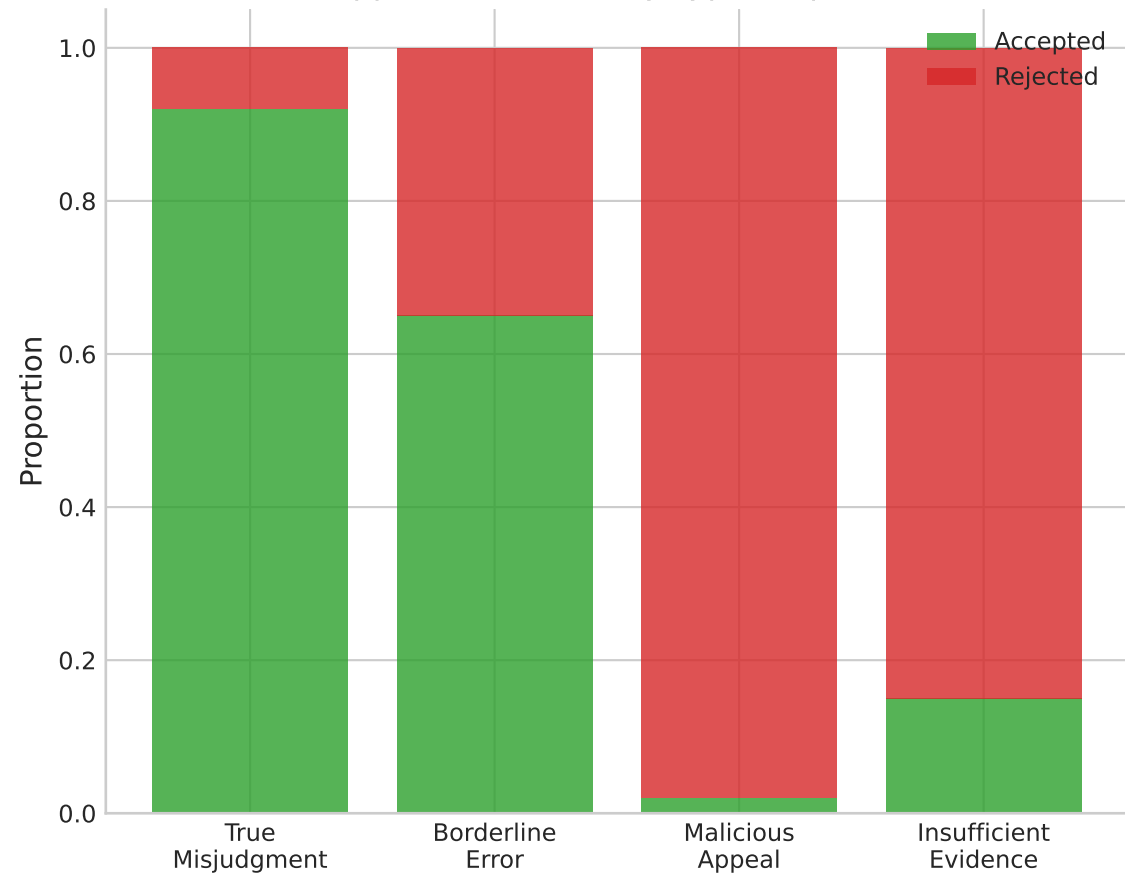
Appeal Outcomes by Type (Exp. 13)
