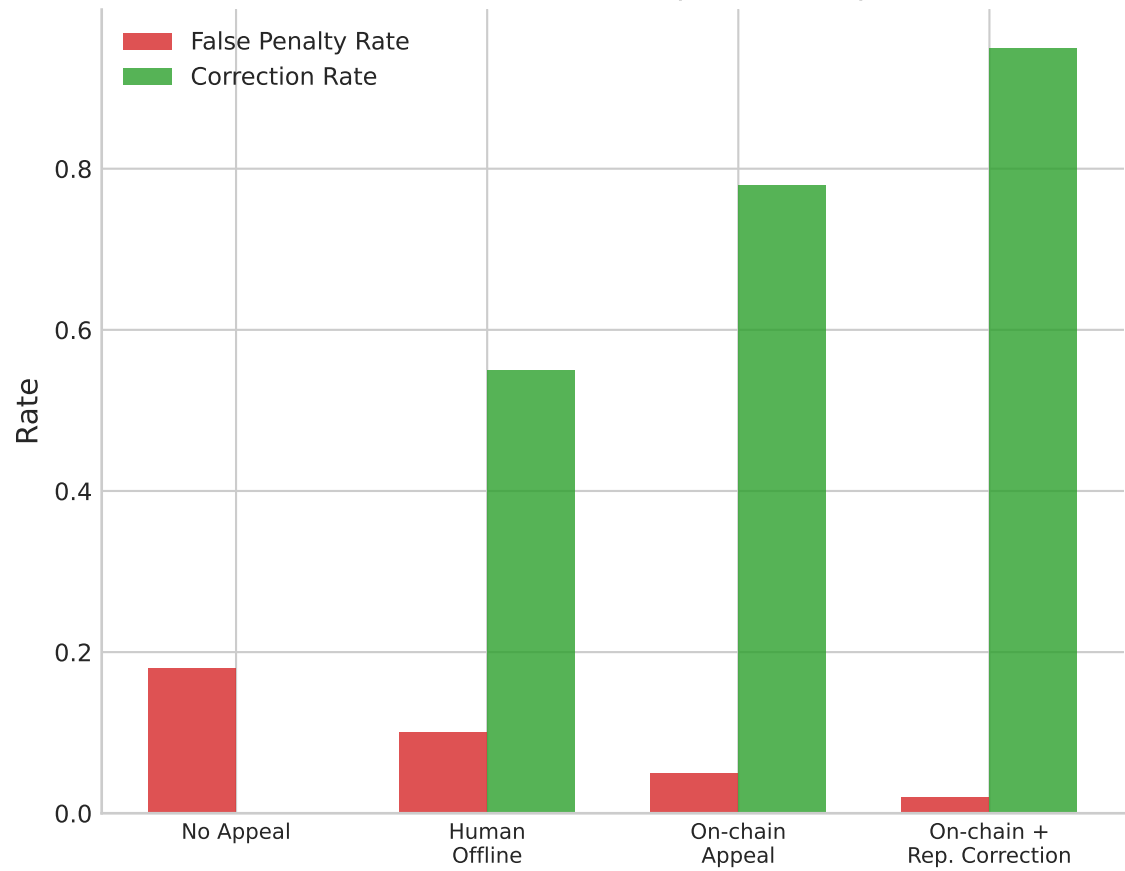
Governance Benefit Comparison (Exp. 14)
