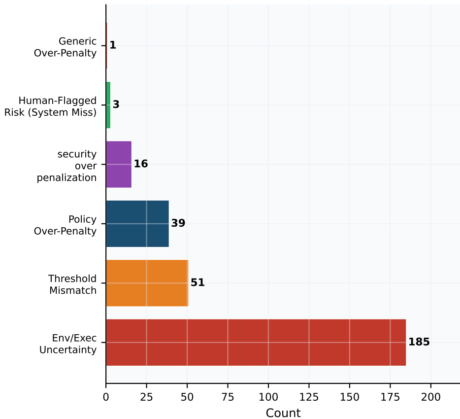
B. Divergence Taxonomy (System-Fail / Human-Pass)
