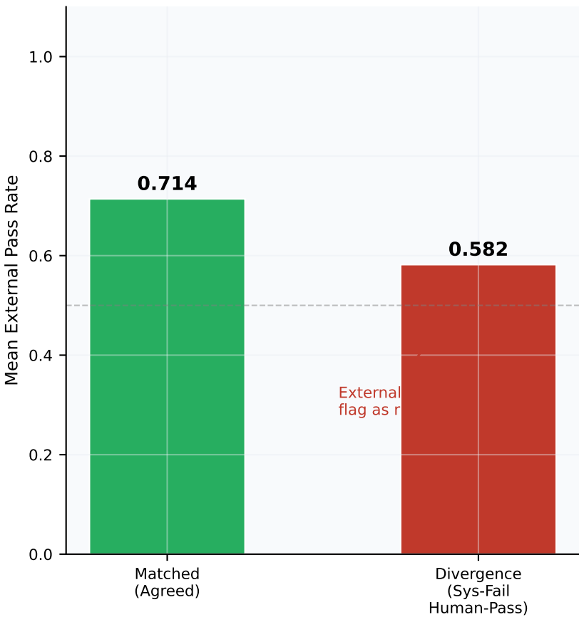
C. External Evaluator Validation (Independent 3rd-party)
