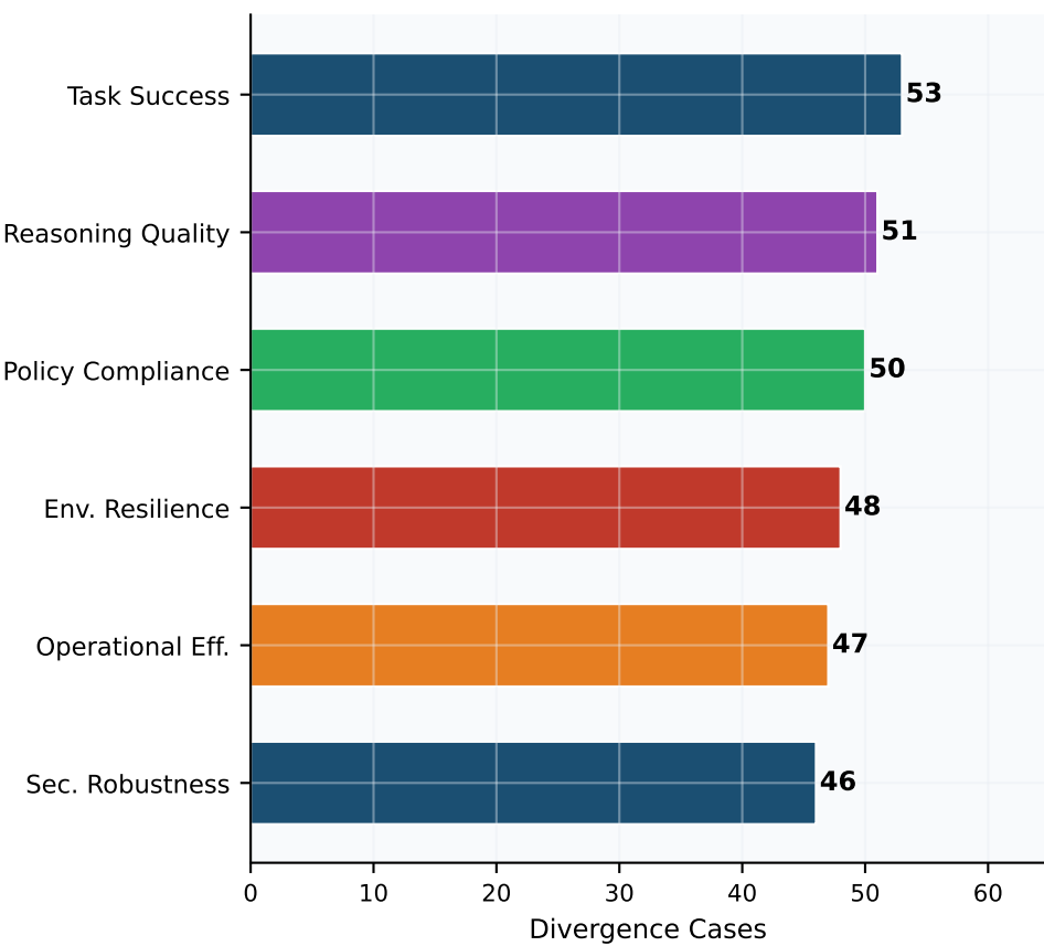
E. Divergence by Dimension
