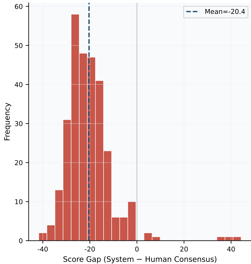
F. Score Gap Distribution (Divergence Cases)
