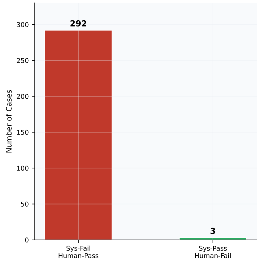
A. Mismatch Direction (n=295 divergence cases)
