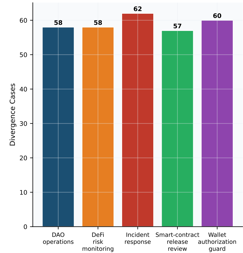
D. Divergence by Domain
