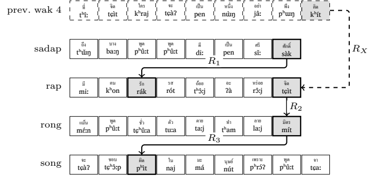
Fig. 1. The example stanza with its rhyme positions shaded and linked: R_1 (sadap→rap), R_2 (rap→rong), R_3 (rong→song); the dashed R_X arrow links the final syllable (k'it) of the previous stanza's wak 4 to wak 2's final syllable (təit).
