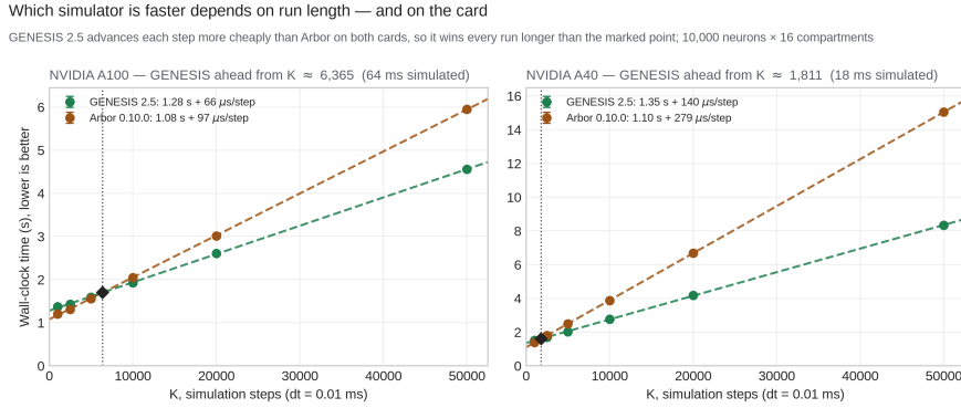
Figure 5: Neither simulator is faster in general: which one wins depends on how long the run is, and where the changeover falls depends on the card. Both are linear in K — Arbor starts about 0.2\text{ s} ahead on setup, GENESIS 2.5 advances each step more cheaply — so a comparison at a single run length reports whichever side of the crossing the author happened to choose. Our per-step margin is the wider one on the A40, 140 against Arbor’s 279\,\mu\text{s} , where on the A100 it is 66 against 97; the crossing moves accordingly, from K \approx 6400 to K \approx 1800 . Our kernel is fp32 where Arbor computes in double, and the A40’s double-precision throughput is a fraction of the A100’s. N = 10\,000 neurons \times 16 compartments, mean \pm std over 3 replicates.
