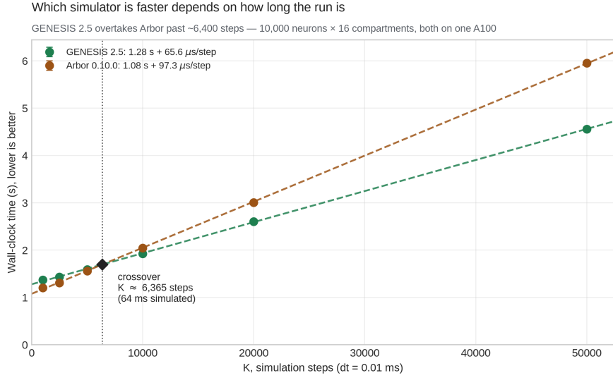
Figure 5: Neither simulator is faster in general: which one wins depends on how long the run is. Both are linear in K — Arbor starts 0.20s ahead on setup, GENESIS 2.5 advances each step 33% more cheaply — so the lines cross at K \approx 6400 , and a comparison at a single run length reports whichever side of that the author happened to choose. Both arms are on the A100, the only card we ran Arbor on. Our own kernel costs 140.6 \mu\text{s} per step on the A40 against 65.6 here, so where the lines cross belongs to this card rather than to the pair of simulators. N = 10\,000 neurons \times 16 compartments, six run lengths, mean \pm std over 3 replicates.
